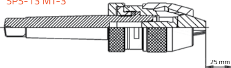
SPS-13 + arbor CM-3
