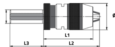
Straight Shank
