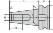
MAS-BT ISO 30/40/50
